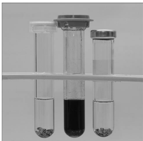
Figure 2. Effect of constant power microwave irradiation (300 W) on stirred Mg turnings in THF (maximum temperature 65 °C) using three single-mode microwave reactors with different field strengths: a) CEM Discover; b) Anton Paar Monowave 300; c) Biotage Initiator EXP 2.5. See main text for discussion.
