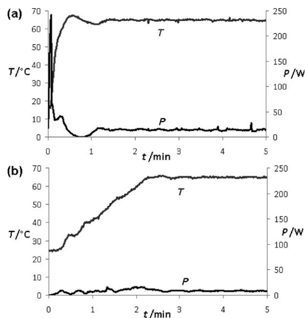
Figure 1. Temperature ( T ) and power ( P ) profiles for the microwave-assisted conversion of 2-chloropyridine ( 1 ) to Grignard reagent 2 (Scheme 1) in temperature-control mode. Monowave 300 reactor, 65°C set temperature, internal fiber-optic temperature control, simultaneous cooling, magnetic stirring (600 rpm). Data are shown using “as-fast-as-possible” (a), and “ramp” modes (b). For clarity, only the first 5 min of the experiment is shown. A simulation of the corresponding electric field strength and volume power distribution at 16 and 240 W microwave power is shown in Figures S5 and S6 in the Supporting Information.
