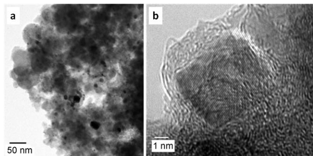
Figure 4. Transmission electron microscopy (TEM) investigation of the fine black carbonaceous powder formed by high field density microwave irradiation of Mg turnings. a) Dark MgO particles are embedded in carbon; b) high resolution TEM image showing a MgO cube with the [100] lattice fringes which is covered by partly graphitized carbon (for further characterization data, see Figures S12–S14 in the Supporting Information).
